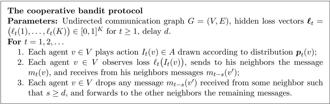
Figure 1: The cooperative bandit protocol where all agents share the same delay parameter d .
